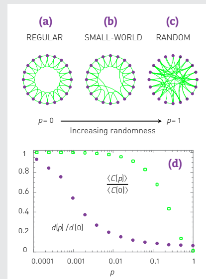
Figure 3.14 The Watts-Strogatz Model
