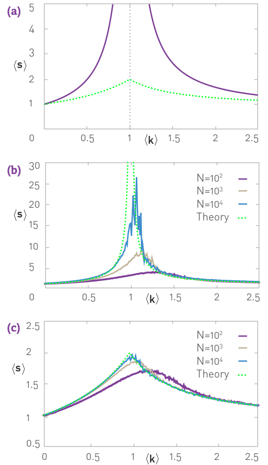
Figure 3.20 Average Component Size
