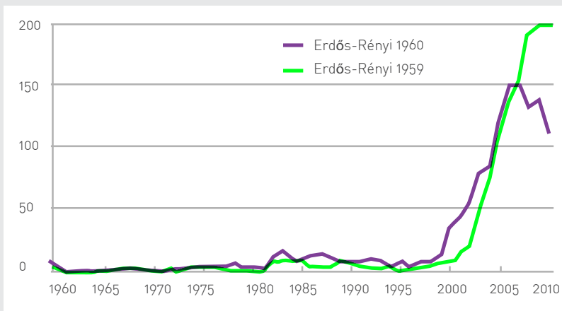
Figure 3.15 Network Science and Random Networks
