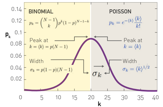
Figure 3.4 Binomial vs. Poisson Degree Distribution
