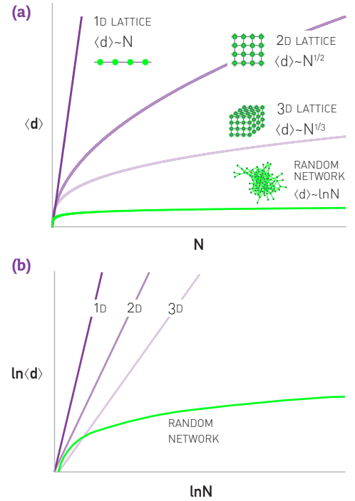
Figure 3.11 Why are Small Worlds Surprising?
