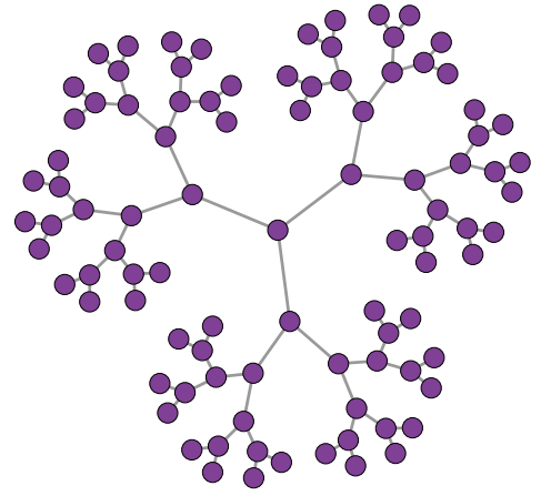
Figure 3.16 Cayley Tree
